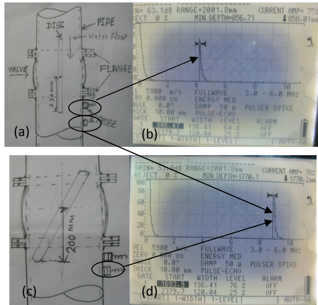
230 mm from the centre of the valve Fig.3, a & c – Probe positions on the downstream of the valve; b- Echo when sensor put within 230 mm of fully open valve; d –Echo when sensor put beyond the flapper disc either full or partial open
