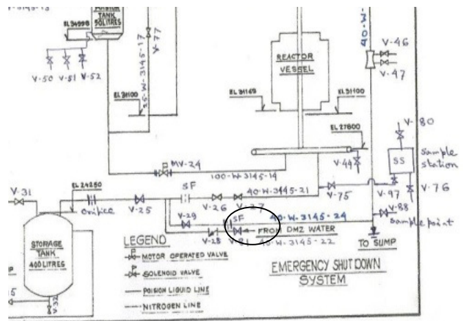
Fig 4. Flow diagram (part) of ESD presence of water in those areas.
