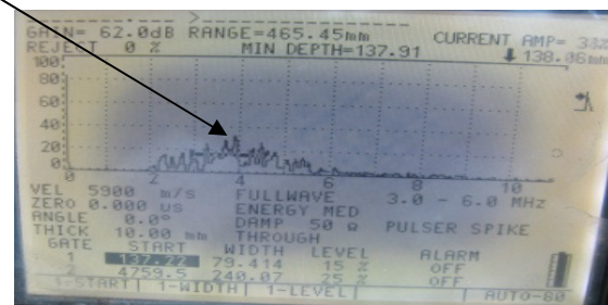
Fig. 6 (c) Echo through sand
